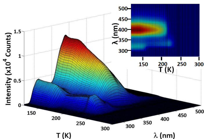
Figure 3. Wavelength-resolved TPD of bilayer of biphenyl and naphthalene for which \Theta_{biphenyl} = 140 ML and \Theta_{naphthalene} = 140 ML. The fluorescence from the two adsorbates are distinguishable. Mixing occurs at about 20 K before desorption. Inset: top view.
