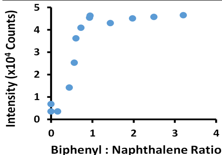
Figure 6. Maximum Intensity of the naphthalene peaks at 325 and 334 nm at T = 210 K in Figure 4 as a function of the ratio of biphenyl to naphthalene coverages. \Theta_{\text{naphthalene}} was held constant at 146 \pm 14 ML.
