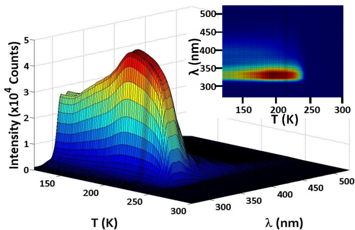
Figure 4. Wavelength-resolved TPD of bilayer of naphthalene and biphenyl, for which \Theta_{\text{naphthalene}} = 140 ML and \Theta_{\text{biphenyl}} = 440 ML. The fluorescence is that of molecular naphthalene with \lambda_{\text{max}} \sim 325 and 334 nm. Note the absence of the 320 nm emission from the twisted conformer of biphenyl. Inset: top view. The excimers of biphenyl and naphthalene are barely visible at 370 and 397 nm, respectively.
