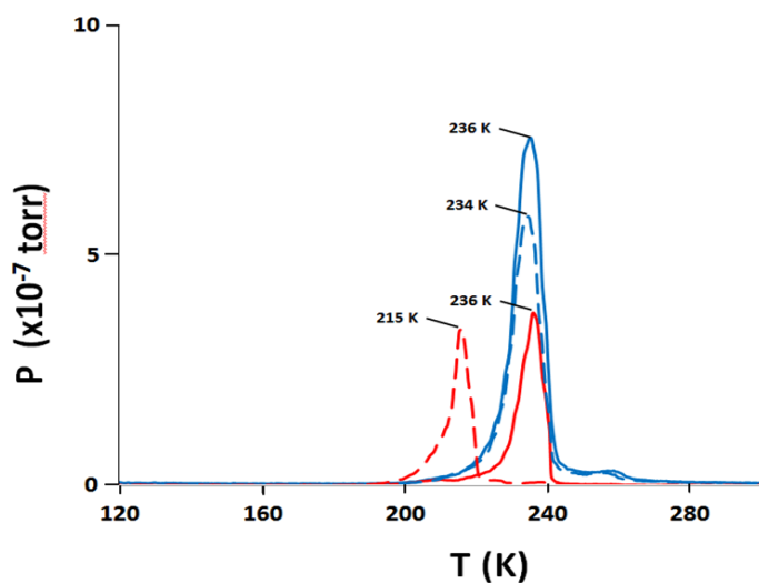
Figure 5. Mass specific TPD for multilayer biphenyl, multilayer naphthalene and biphenyl and naphthalene in the bilayer. T_p 's for pure naphthalene (red, dashed plot) and pure biphenyl (blue, dashed plot) are 215 and 234 K, respectively. In the bilayer, T_p 's for naphthalene (red, solid plot) and biphenyl (blue, solid plot) are both 236 K.
