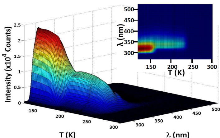
Figure 1. Wavelength-resolved TPD of multilayer biphenyl. \Theta_{biphenyl} = 340 ML. Biphenyl deposited in the twisted conformation with \lambda_{max} \sim 320 nm that red-shifts to 340 nm subsequent to the disorder-to-order transition. Inset: top view.
