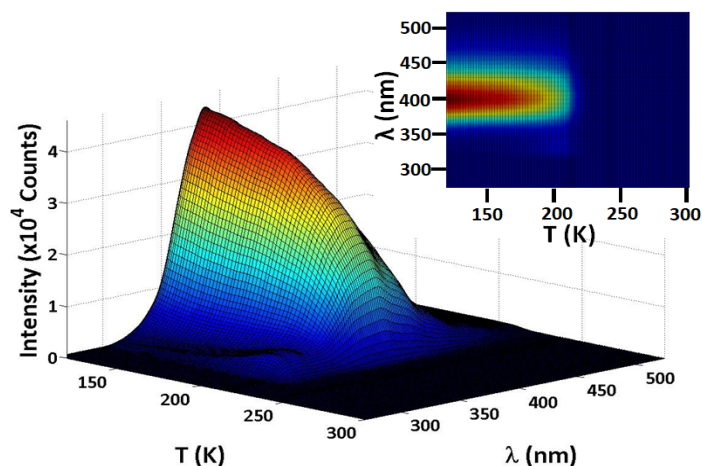
Figure 2. Wavelength-resolved TPD of multilayer naphthalene \Theta_{naphthalene} = 120 ML. The excimer fluorescence at \lambda_{max} \sim 395 nm dominate at deposition that blue-shifts to 325 nm subsequent to the disorder-to-order transition. Inset: top view.
